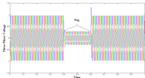
3-Ø Voltage at Load Point, With 3-Ø Fault, Without DVR
