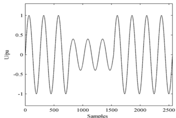
Fig. 1.1: Voltage Dip (Sag) Waveform
