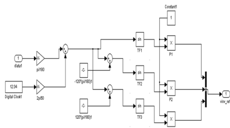
Fig. Firing Angle Controller Scheme
