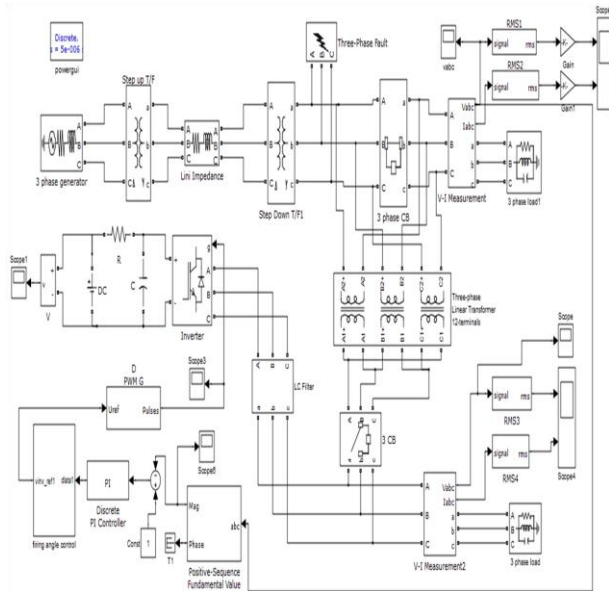
Simulink Model of DVR in Power System
