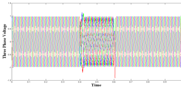
3-Ø Voltage at Load Point, With 3-Ø Fault, With DVR
