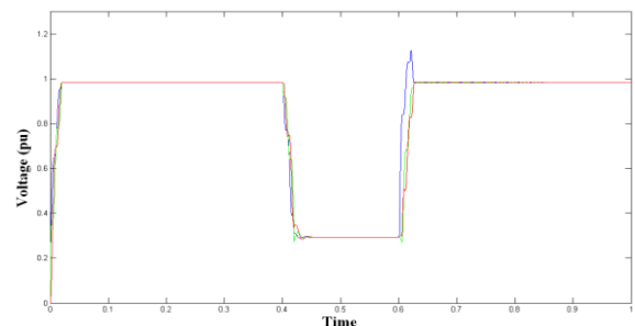
P.U Voltage at Load Point, With 3-Ø Fault, Without DVR
