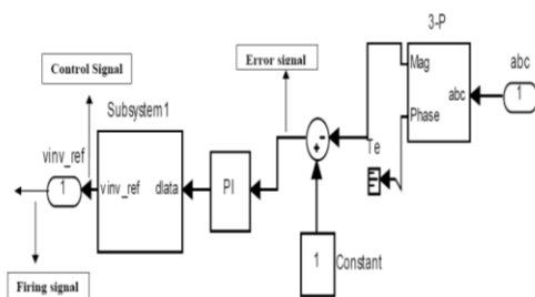
Fig 2. SIMULINK Model of DVR Controller
