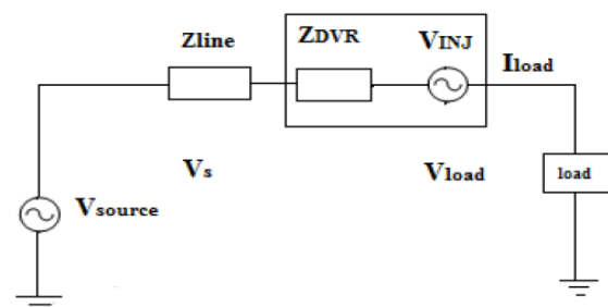
Equivalent Circuit Diagram of DVR
