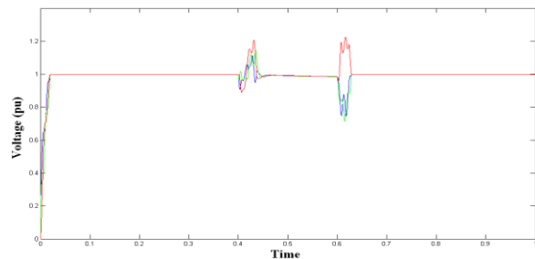
P.U Voltage at Load Point, With 3-Ø Fault, With DVR
