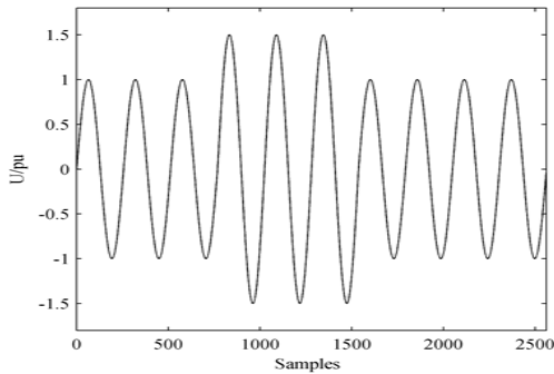
Fig. 1.2: Voltage Swell Waveform
